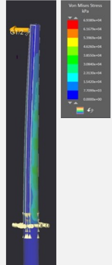
Calculated strength
